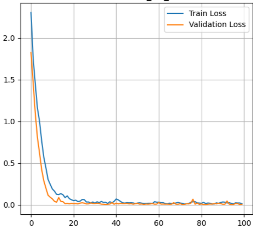
Loss: FCovSel_SG_MSC
